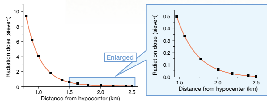
This figure shows relationship between distance from the hypocenter and air dose (without shielding), according to DS02. When a person is exposed to radiation in a typical Japanese house, radiation decreases to half of the doses presented here.
